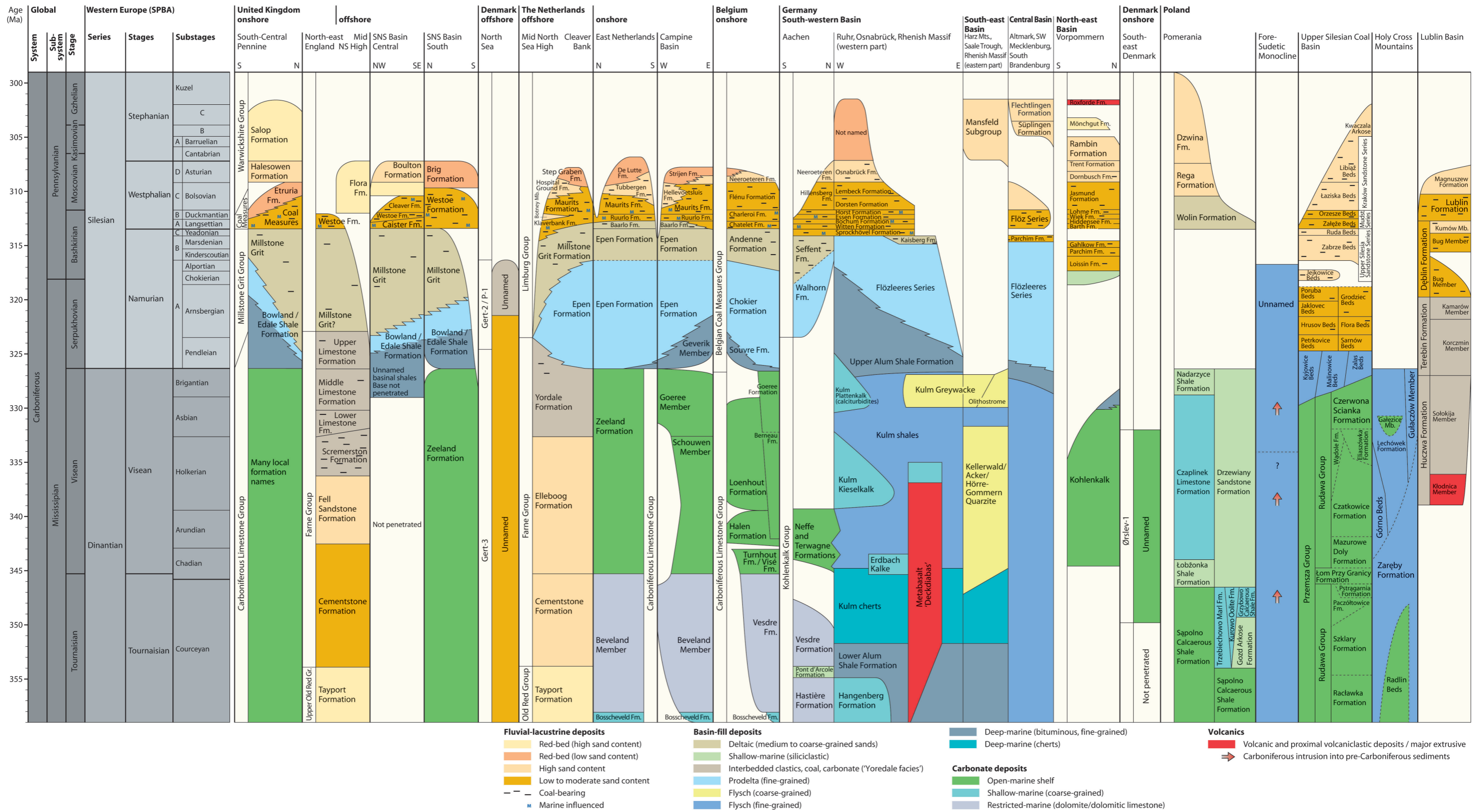
Figure 6.3. Carboniferous lithostratigraphy in the SPBA area. Based on Michelsen (1971), Bertelsen (1972), Cameron (1993), Delmer et al. (2001), Poty et al. (2001), Menning & Hendrich (2002), Besly (2005), Collinson (2005), Van Buggenum & Den Hartog Jager (2007), Wagner (2007).
