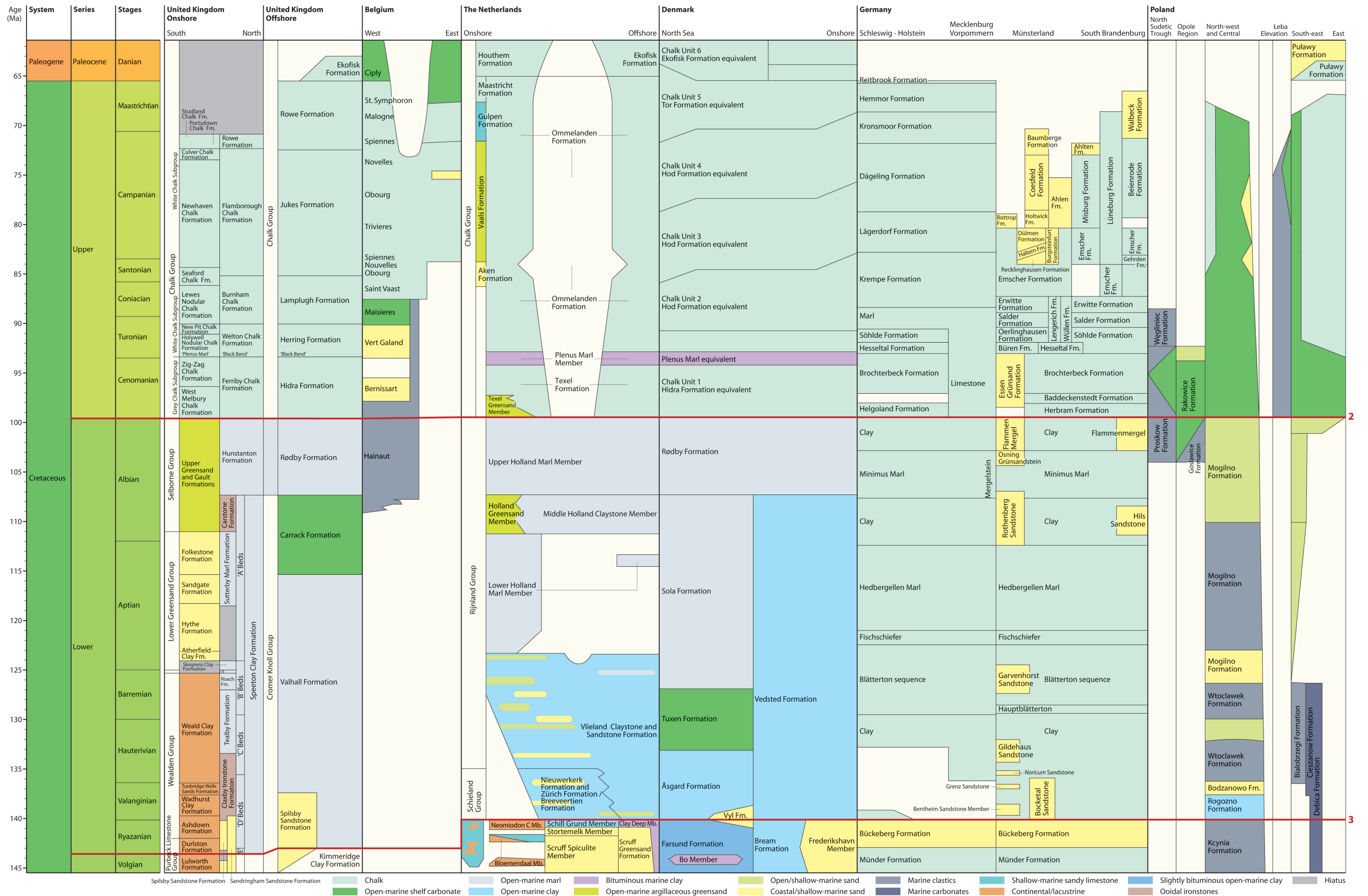
Figure 11.1. Tectonostratigraphic chart of the Cretaceous. The red lines at the base of the Cenomanian (2) and Ryazanian (3) are the lithostratigraphic horizons used to map the depths to the base of the Upper Cretaceous and near the base of the Ryazanian. See Figures 1.5, 11.2 & 11.3.
